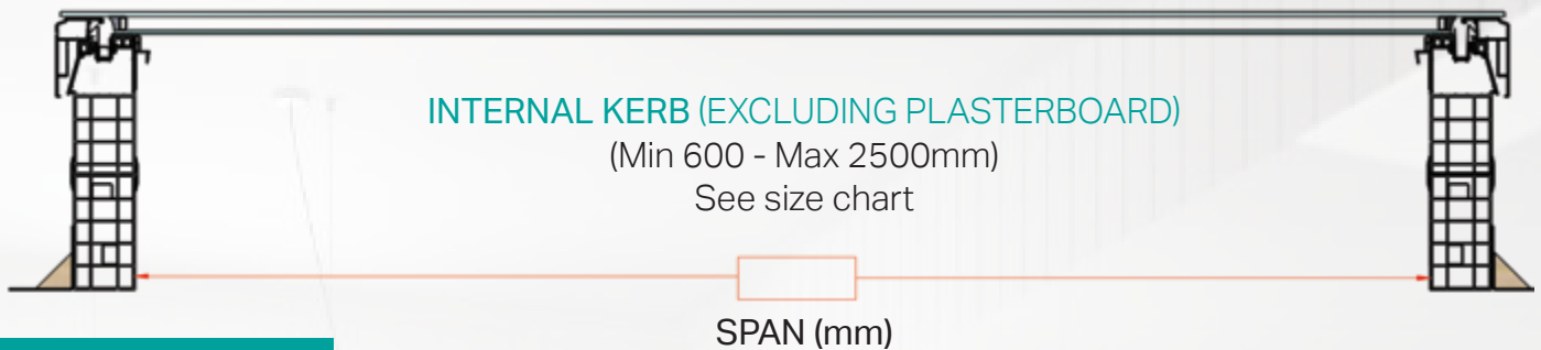
FRONT ELEVATION
